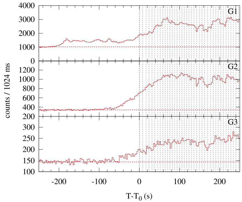
Konus-WIND S1 SOL2002-10-20T14:25 (M1.8) T 0 = 51939.884 s UT (14:25:39.884)
