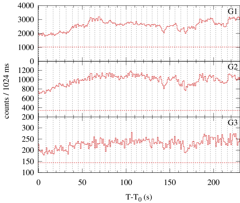
Konus-WIND S1 SOL2002-10-20T14:25 (M1.8) T 0 = 51939.884 s UT (14:25:39.884)
