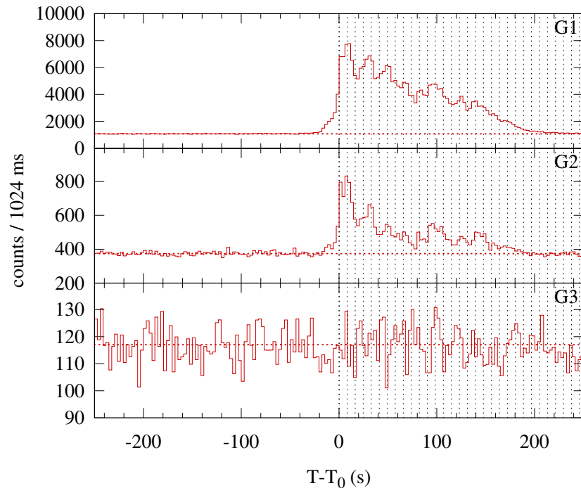
Konus-WIND S2 SOL2002-10-22T15:32 (M1.0) T 0 = 55935.604 s UT (15:32:15.604)
