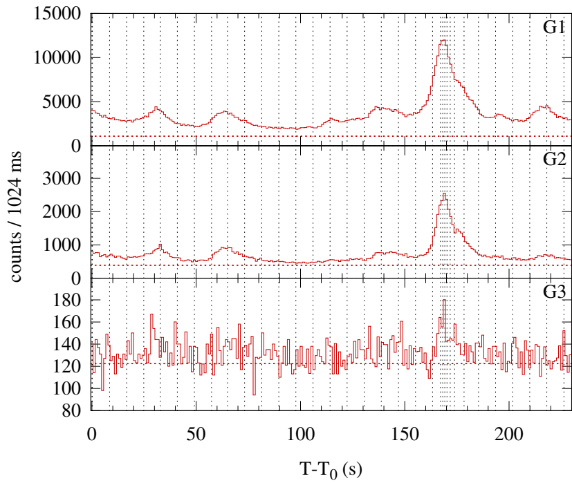
Konus-WIND S2 SOL2002-11-09T13:13 (M4.6) T_0 = 47623.632 s UT (13:13:43.632)
