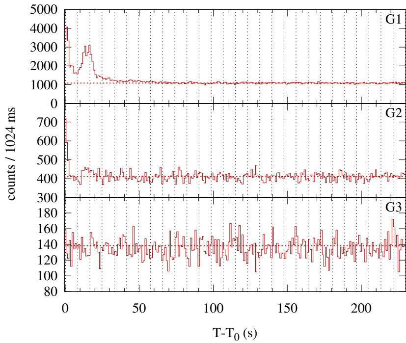
Konus-WIND S2 SOL2002-12-20T20:13 (C7.2) T 0 = 72793.218 s UT (20:13:13.218)
