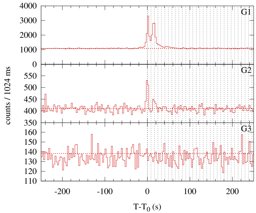
Konus-WIND S2 SOL2002-12-20T20:13 (C7.2) T 0 = 72793.218 s UT (20:13:13.218)
