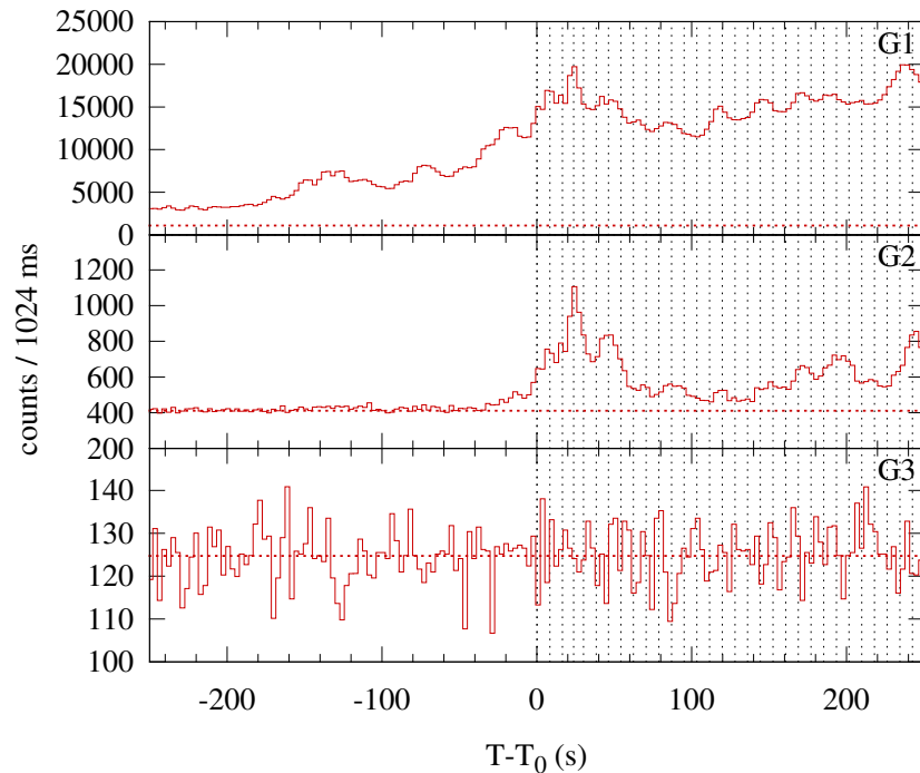
Konus-WIND S2 SOL2003-03-18T12:01 (X1.5) T_0 = 43285.977 s UT (12:01:25.977)
