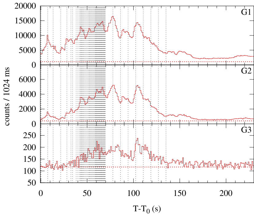
Konus-WIND S2 SOL2003-04-21T13:03 (M2.8) T_0 = 46987.723 s UT (13:03:07.723)
