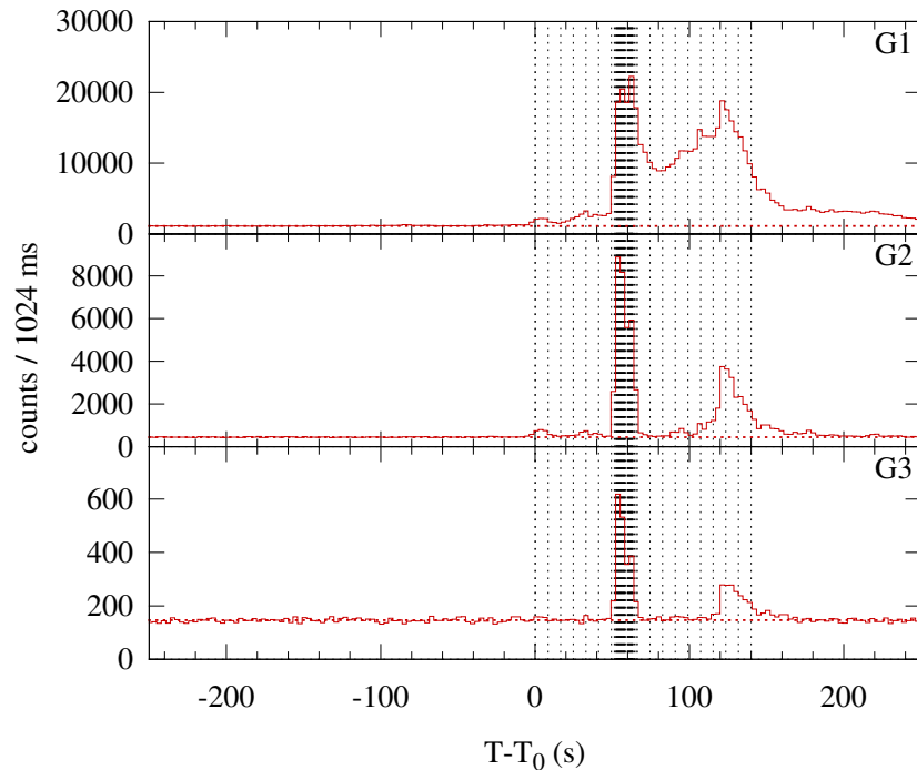
Konus-WIND S2 SOL2003-04-26T08:04 (M7.0) T_0 = 29074.478 s UT (08:04:34.478)
