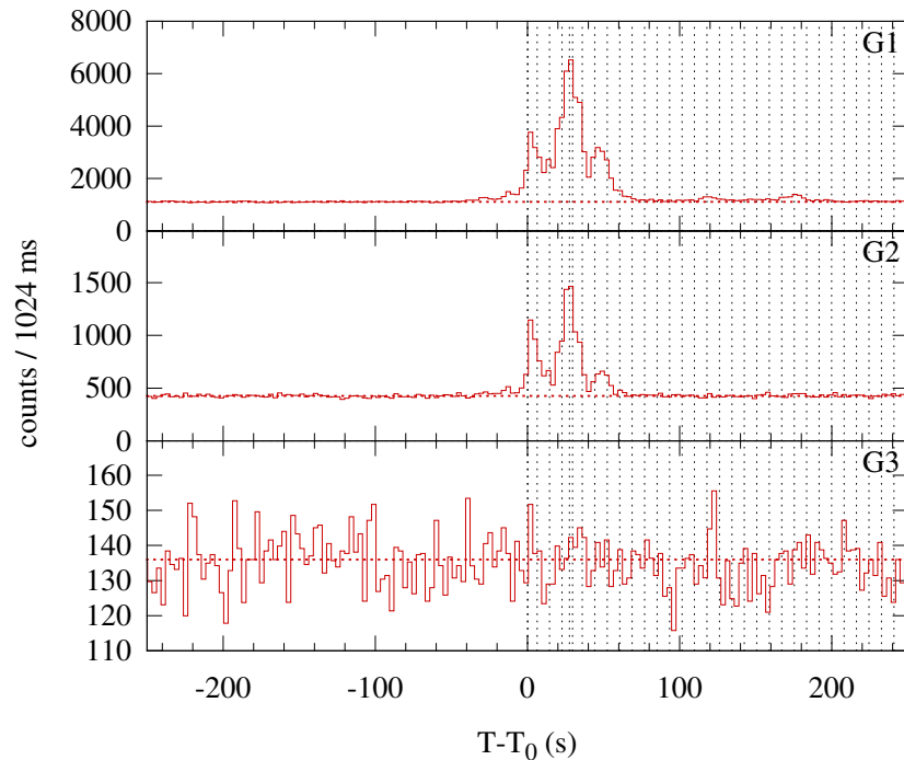
Konus-WIND S2 SOL2003-04-27T07:38 (C8.1) T 0 = 27516.283 s UT (07:38:36.283)
