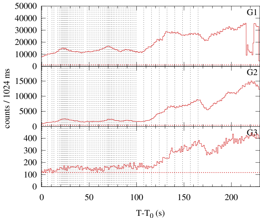
Konus-WIND S2 SOL2003-05-31T02:18 (M9.3) T_0 = 8337.612 s UT (02:18:57.612)
