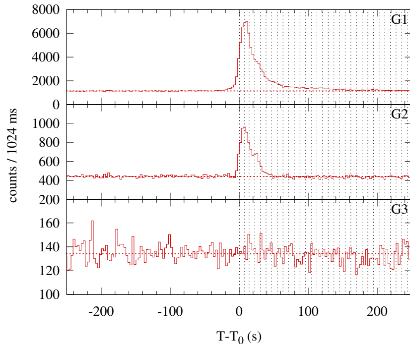
Konus-WIND S2 SOL2003-06-02T13:15 (M1.0) T 0 = 47735.41 s UT (13:15:35.41)
