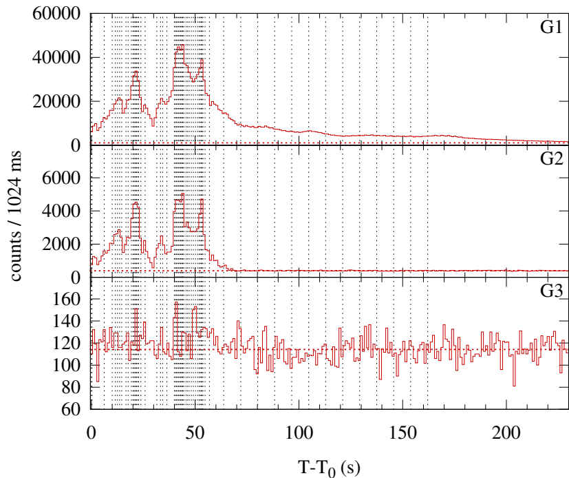
Konus-WIND S2 SOL2003-06-08T16:08 (M4.0) T 0 = 58106.203 s UT (16:08:26.203)
