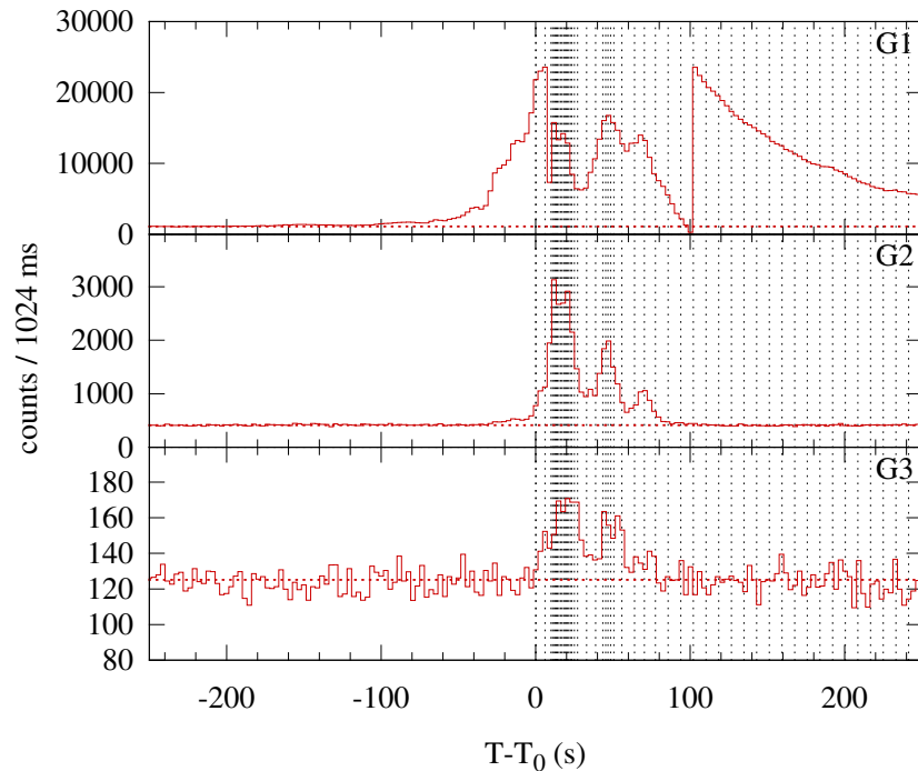
Konus-WIND S2 SOL2003-06-09T21:36 (X1.7) T 0 = 77784.407 s UT (21:36:24.407)
