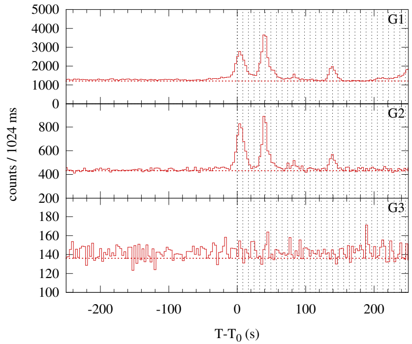
Konus-WIND S2 SOL2003-06-10T11:06 (M5.1) T_0 = 39977.589 s UT (11:06:17.589)
