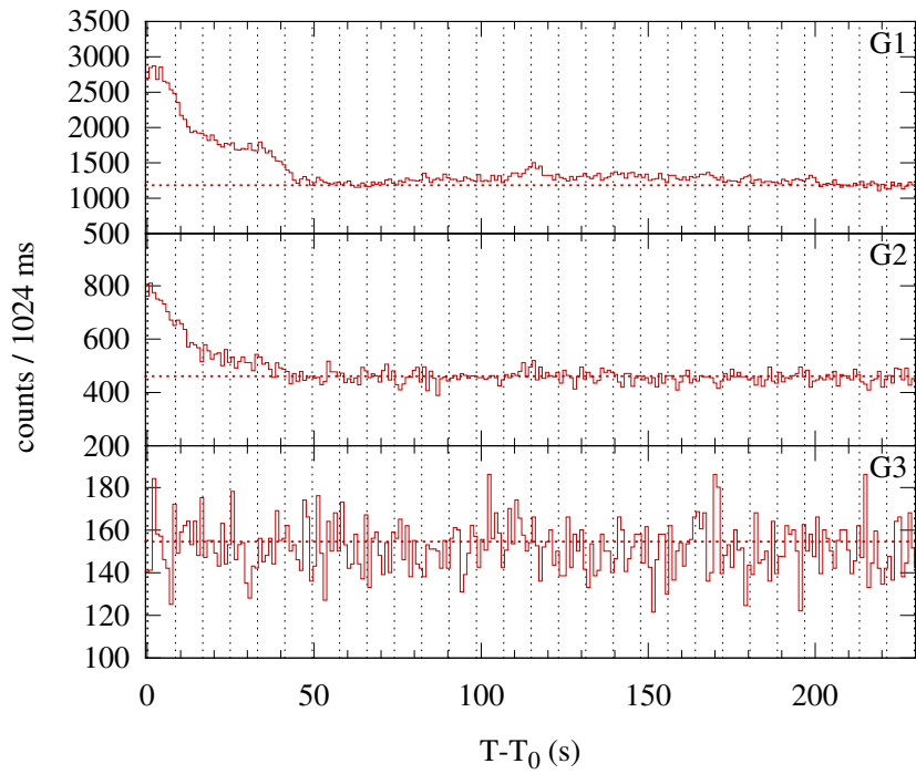
Konus-WIND S2 SOL2003-06-10T16:21 (M1.0) T 0 = 58868.350 s UT (16:21:08.350)
