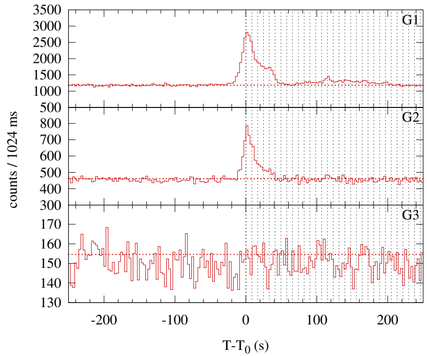
Konus-WIND S2 SOL2003-06-10T16:21 (M1.0) T 0 = 58868.350 s UT (16:21:08.350)
