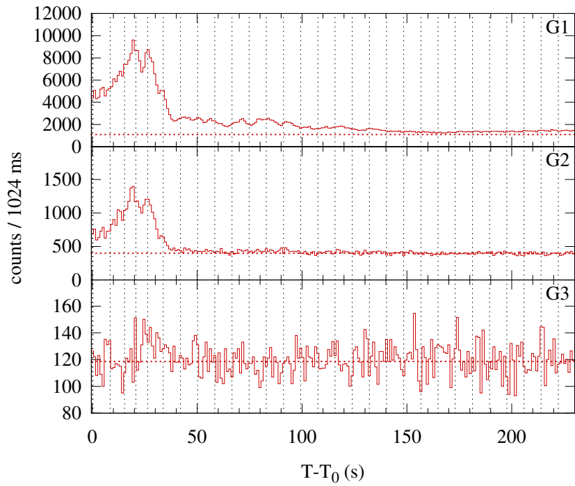
Konus-WIND S2 SOL2003-06-13T04:34 (M1.7) T 0 = 16444.922 s UT (04:34:04.922)
