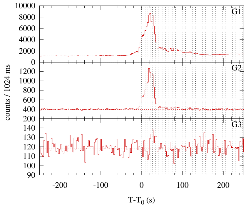
Konus-WIND S2 SOL2003-06-13T04:34 (M1.7) T 0 = 16444.922 s UT (04:34:04.922)
