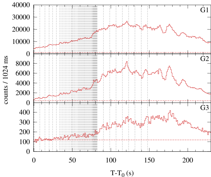
Konus-WIND S2 SOL2003-06-15T23:42 (X1.3) T_0 = 85339.414 s UT (23:42:19.414)
