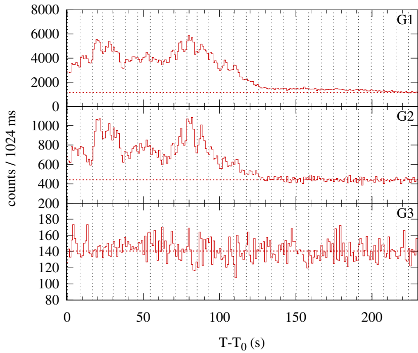
Konus-WIND S2 SOL2003-06-17T21:49 (C5.2) T_0 = 78574.67 s UT (21:49:34.67)
