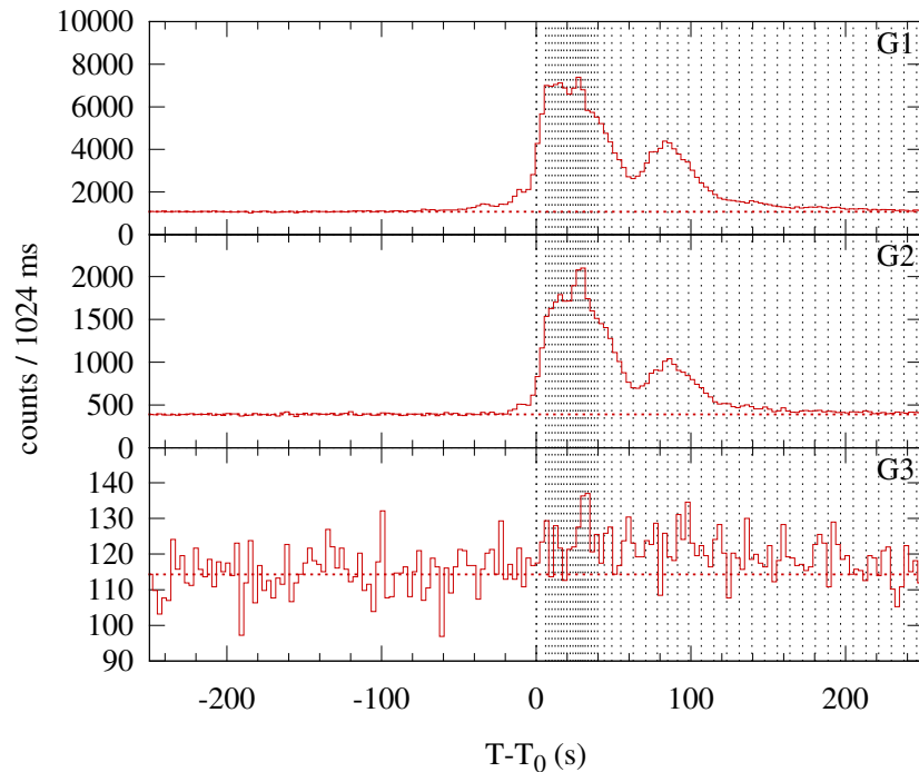
Konus-WIND S2 SOL2003-07-17T08:19 (C9.8) T_0 = 29968.782 s UT (08:19:28.782)
