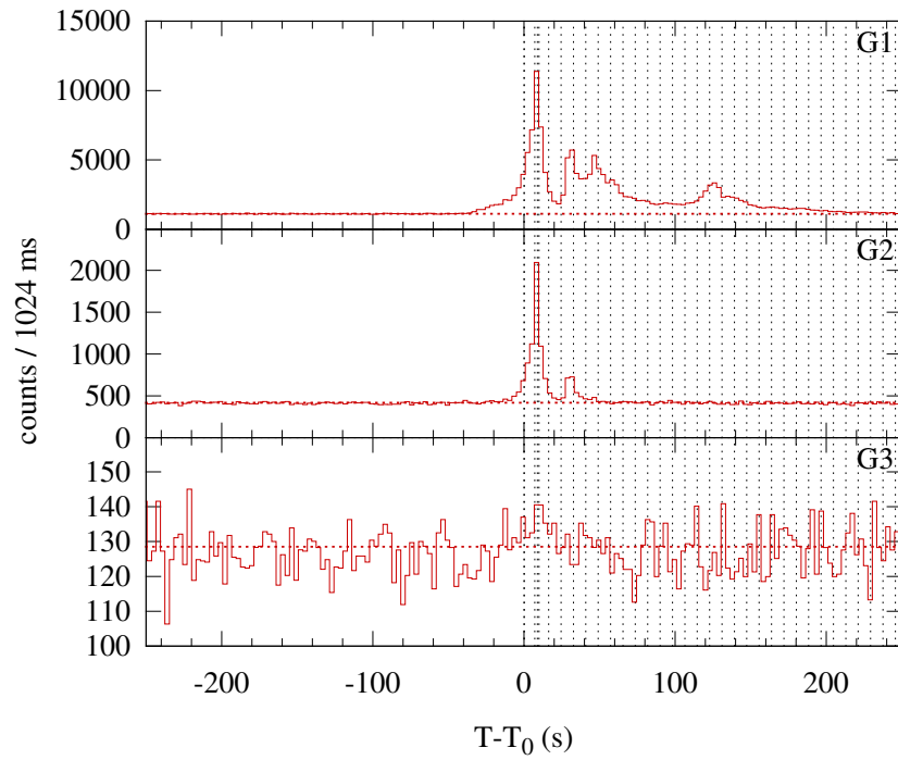
Konus-WIND S2 SOL2003-10-21T08:23 (M1.0) T_0 = 30232.83 s UT (08:23:52.83)
