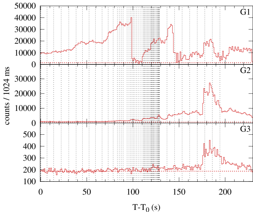
Konus-WIND S2 SOL2003-10-23T08:22 (X5.4) T_0 = 30144.671 s UT (08:22:24.671)
