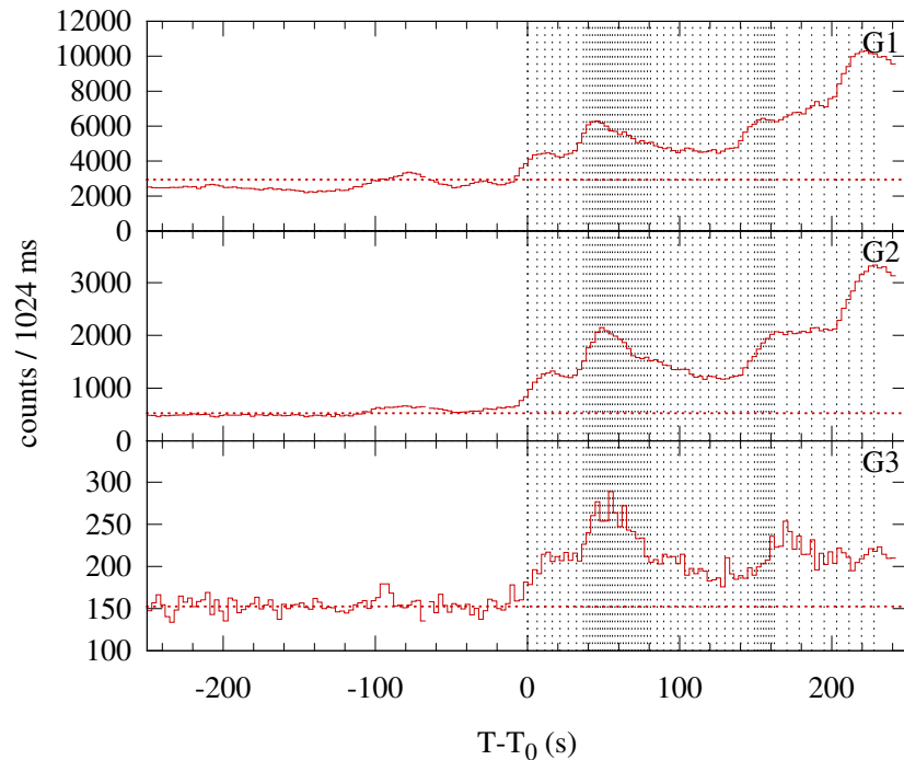
Konus-WIND S2 SOL2003-10-24T02:44 (M7.6) T_0 = 9891.839 s UT (02:44:51.839)
