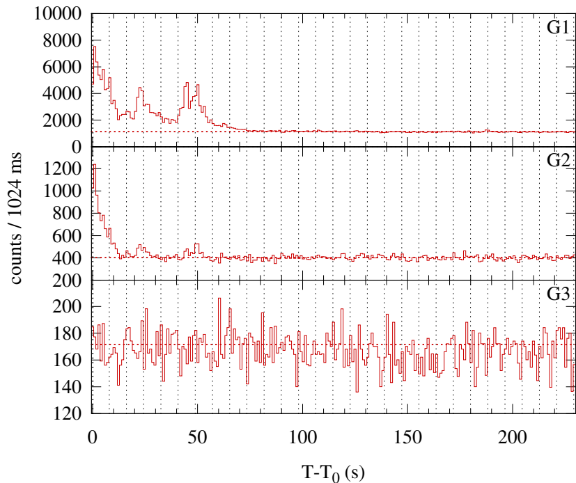
Konus-WIND S1 SOL2003-10-24T10:34 (C9.1) T 0 = 38067.588 s UT (10:34:27.588)
