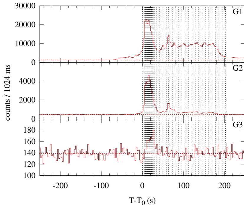
Konus-WIND S2 SOL2003-10-25T10:29 (M1.5) T_0 = 37773.236 s UT (10:29:33.236)
