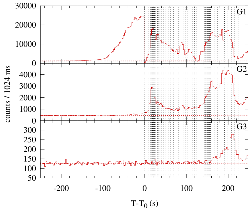
Konus-WIND S2 SOL2003-10-26T06:11 (X1.2) T_0 = 22285.91 s UT (06:11:25.91)
