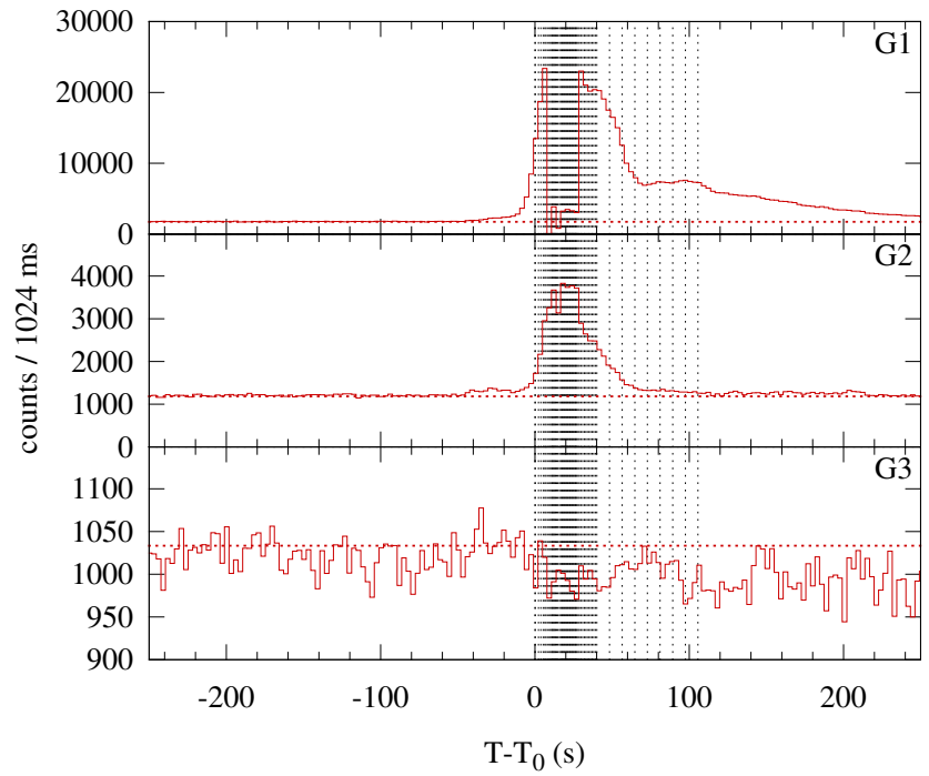
Konus-WIND S2 SOL2003-10-27T09:22 (M5.0) T 0 = 33776.444 s UT (09:22:56.444)
