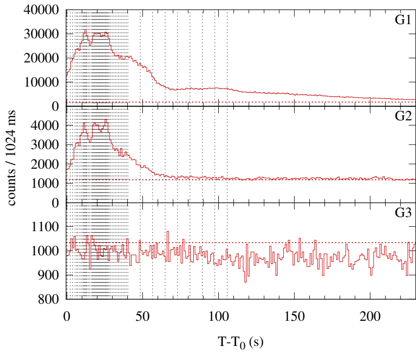
Konus-WIND S2 SOL2003-10-27T09:22 (M5.0) T 0 = 33776.444 s UT (09:22:56.444)
