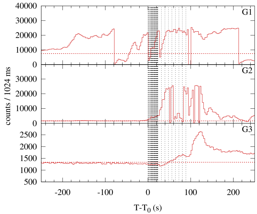
Konus-WIND S2 SOL2003-11-02T17:15 (X8.3) T_0 = 62107.985 s UT (17:15:07.985)
