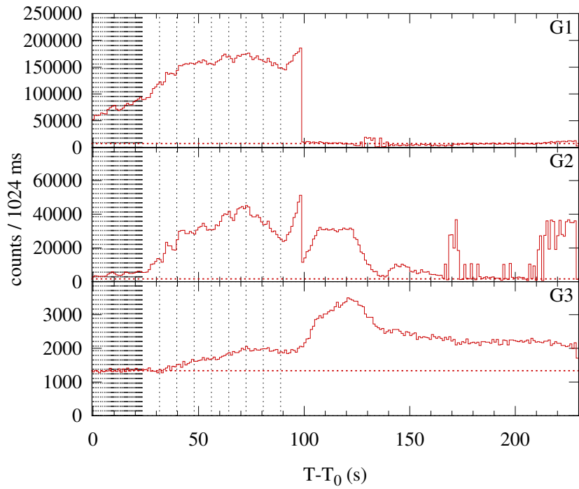
Konus-WIND S2 SOL2003-11-02T17:15 (X8.3) T_0 = 62107.985 s UT (17:15:07.985)
