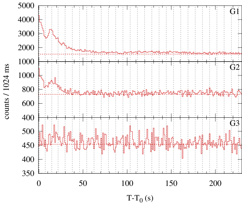
Konus-WIND S2 SOL2003-11-13T05:00 (M1.6) T 0 = 18040.84 s UT (05:00:40.84)
