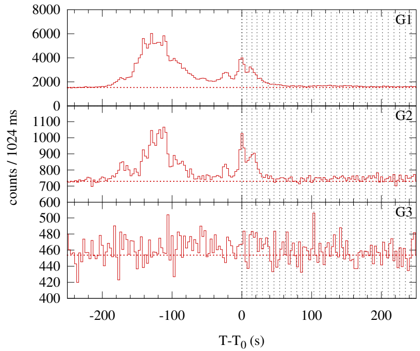
Konus-WIND S2 SOL2003-11-13T05:00 (M1.6) T 0 = 18040.84 s UT (05:00:40.84)
