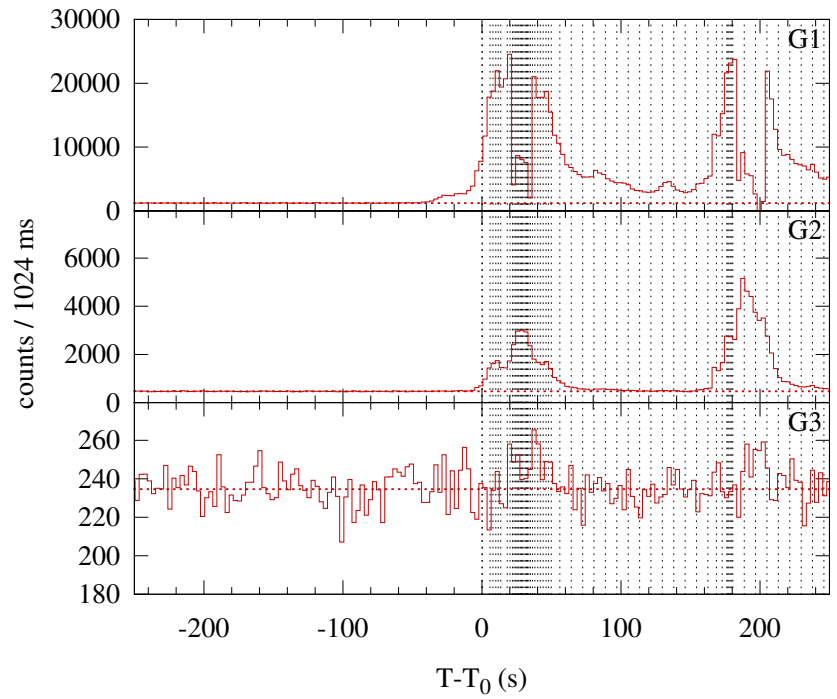
Konus-WIND S2 SOL2003-11-17T08:58 (M4.2) T 0 = 32322.158 s UT (08:58:42.158)
