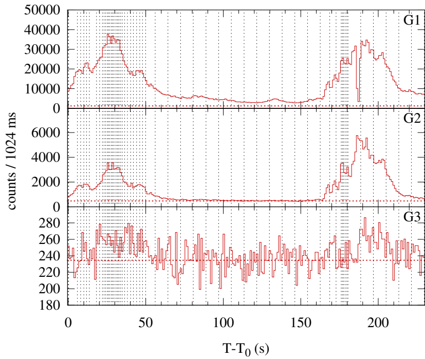
Konus-WIND S2 SOL2003-11-17T08:58 (M4.2) T 0 = 32322.158 s UT (08:58:42.158)
