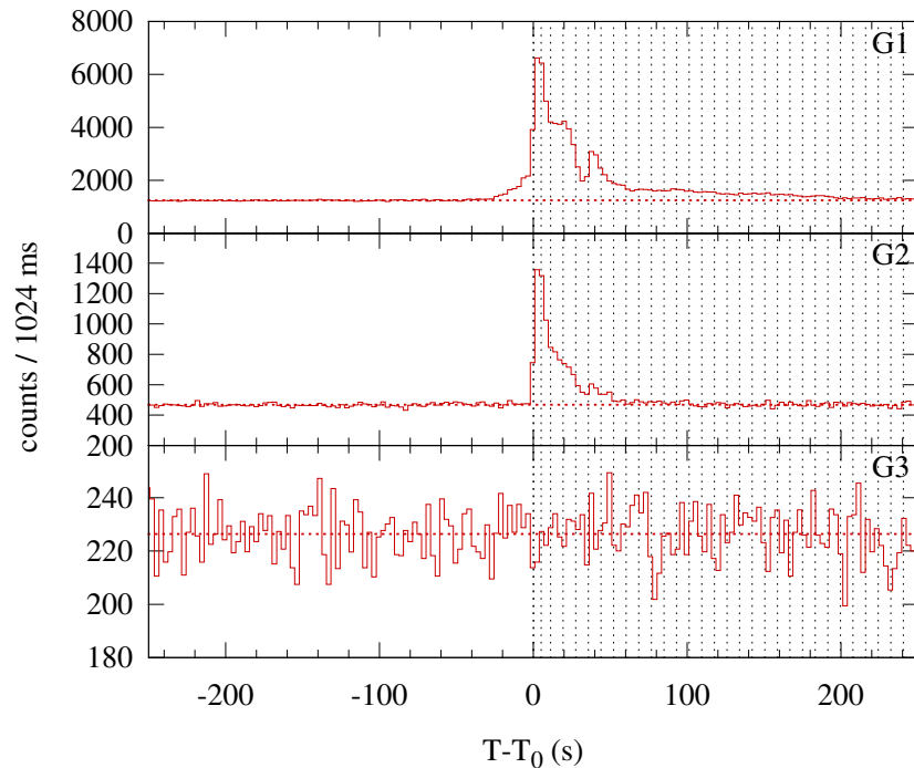
Konus-WIND S2 SOL2003-11-18T01:35 (M1.8) T 0 = 5758.703 s UT (01:35:58.703)
