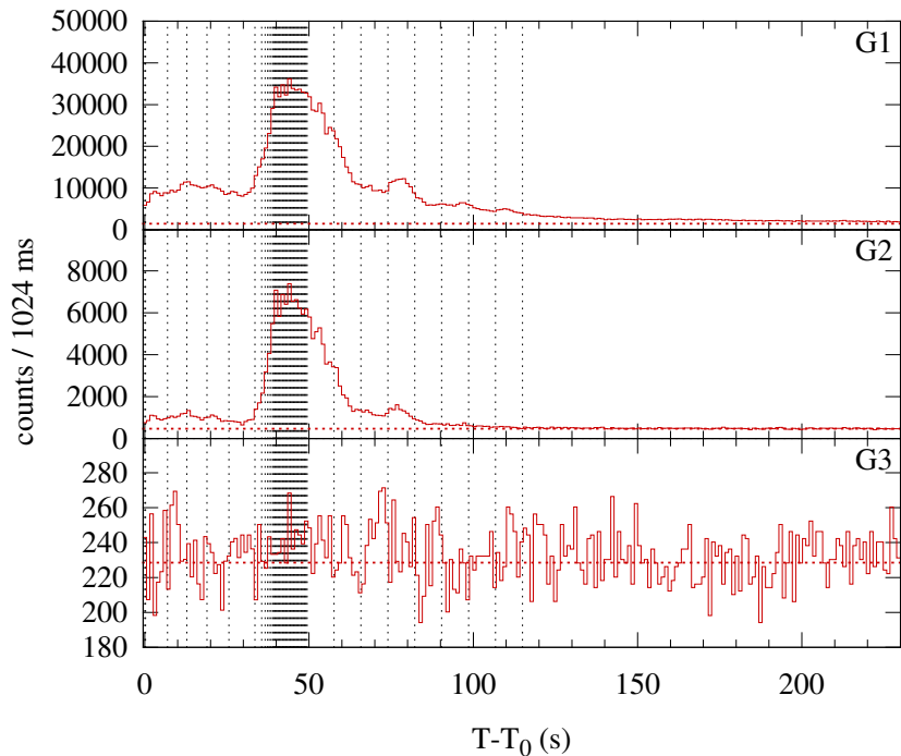
Konus-WIND S2 SOL2003-11-18T07:41 (M3.2) T 0 = 27676.43 s UT (07:41:16.43)
