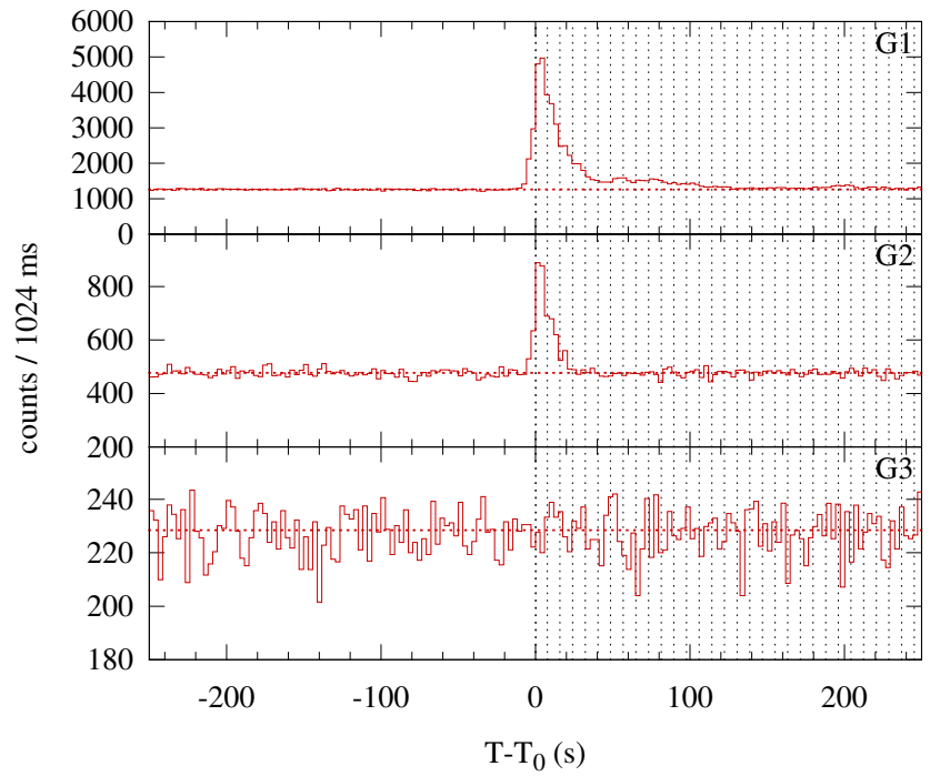
Konus-WIND S2 SOL2003-11-18T22:17 (C6.1) T_0 = 80263.449 s UT (22:17:43.449)
