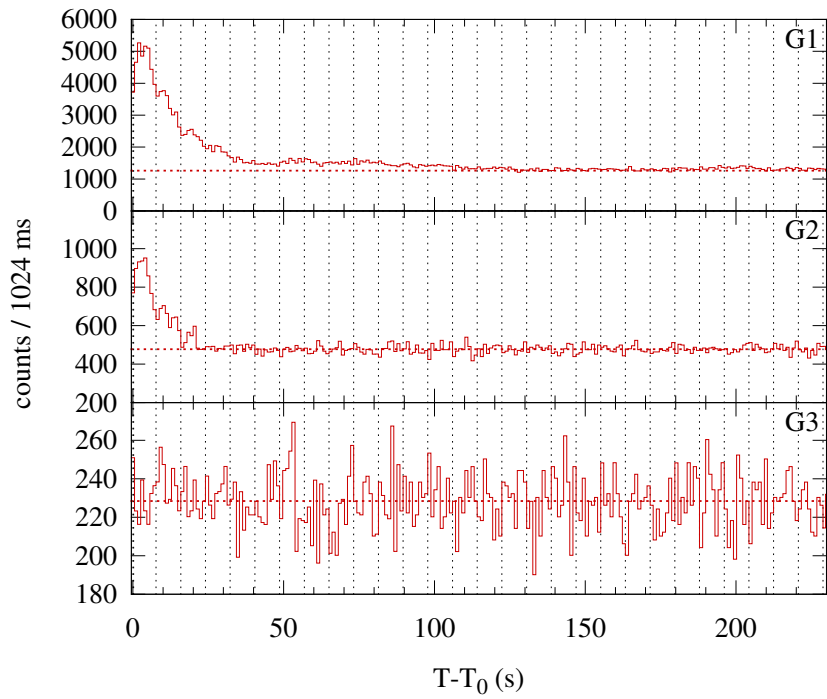
Konus-WIND S2 SOL2003-11-18T22:17 (C6.1) T_0 = 80263.449 s UT (22:17:43.449)
