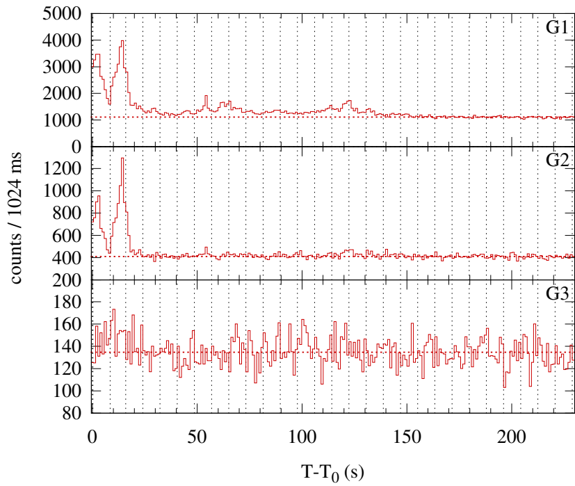
Konus-WIND S2 SOL2003-12-31T18:22 (M1.0) T 0 = 66144.545 s UT (18:22:24.545)
