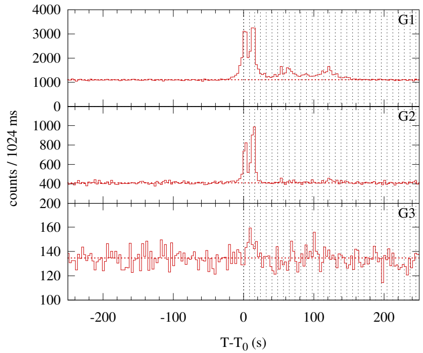
Konus-WIND S2 SOL2003-12-31T18:22 (M1.0) T 0 = 66144.545 s UT (18:22:24.545)
