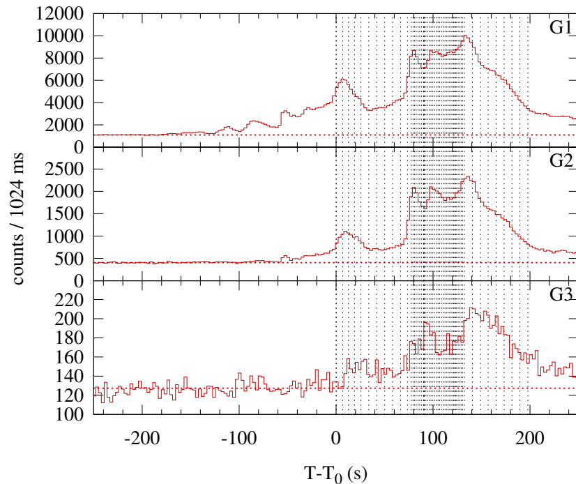
Konus-WIND S2 SOL2004-01-07T10:20 (M8.3) T_0 = 37237.908 s UT (10:20:37.908)
