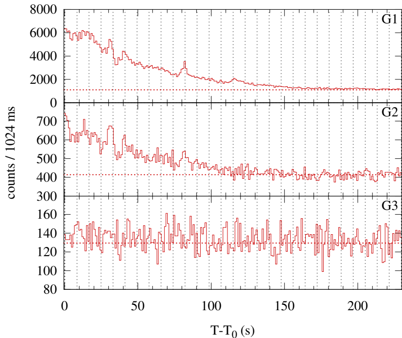
Konus-WIND S2 SOL2004-01-09T01:19 (M1.1) T_0 = 4774.166 s UT (01:19:34.166)
