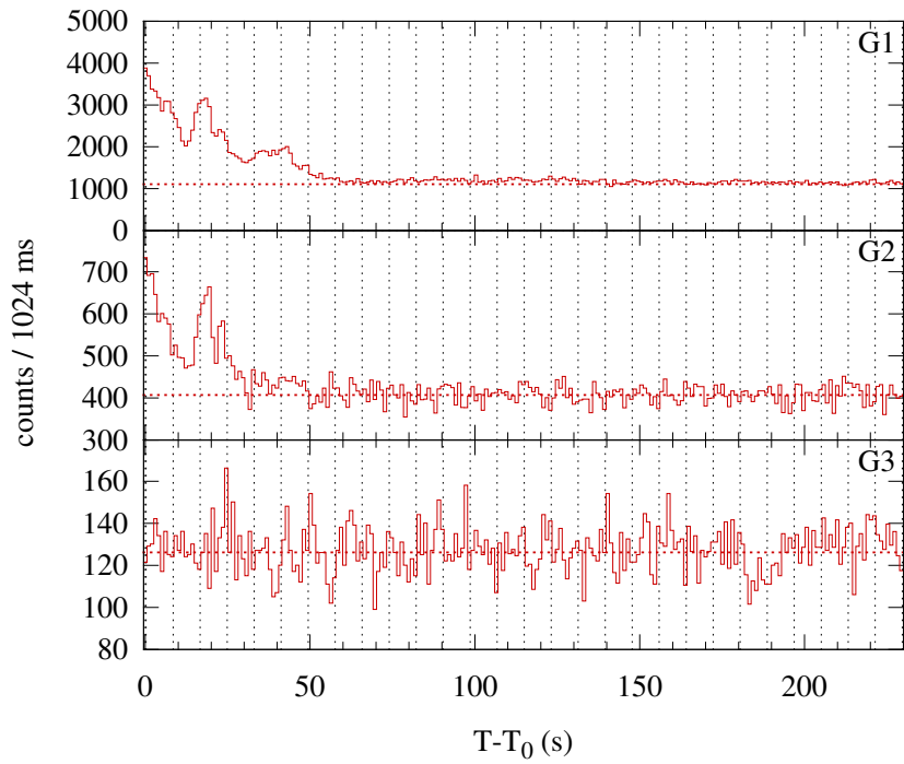
Konus-WIND S2 SOL2004-03-29T19:58 (C4.5) T_0 = 71889.140 s UT (19:58:09.140)
