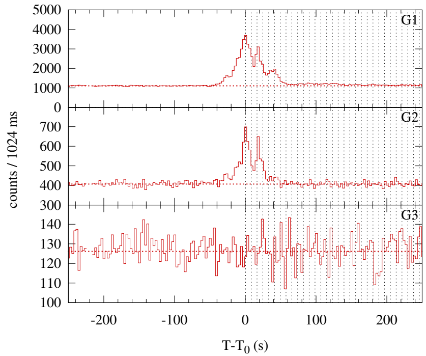
Konus-WIND S2 SOL2004-03-29T19:58 (C4.5) T_0 = 71889.140 s UT (19:58:09.140)
