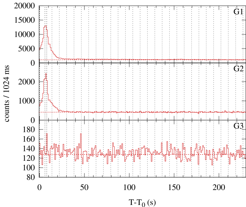
Konus-WIND S2 SOL2004-03-31T20:05 (C7.4) T_0 = 72332.654 s UT (20:05:32.654)
