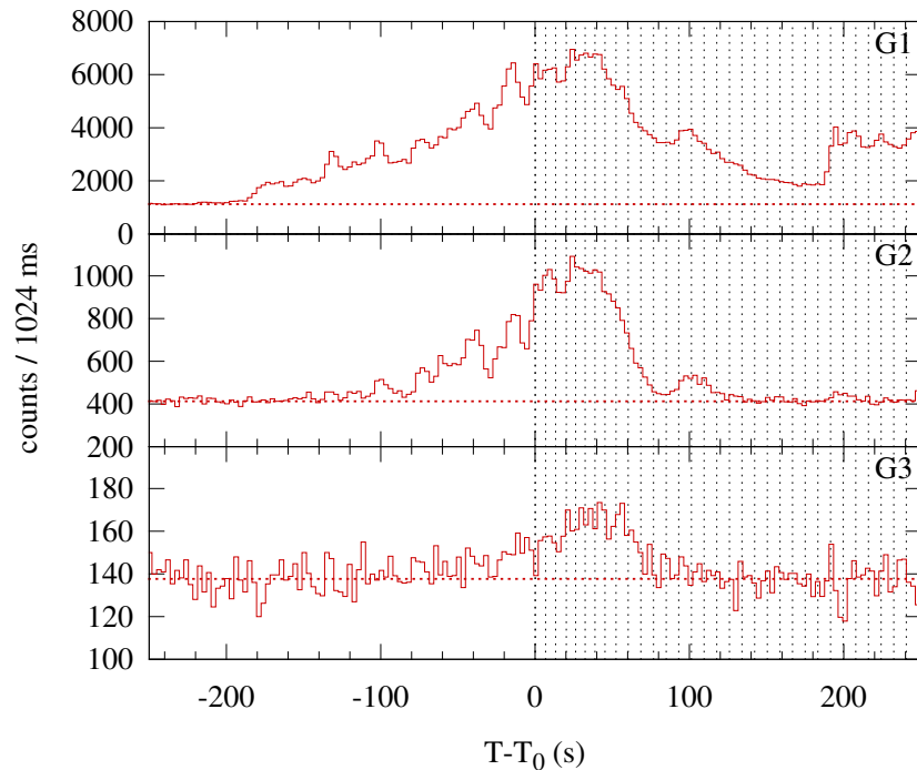
Konus-WIND S2 SOL2004-07-13T08:46 (M5.4) T_0 = 31607.529 s UT (08:46:47.529)
