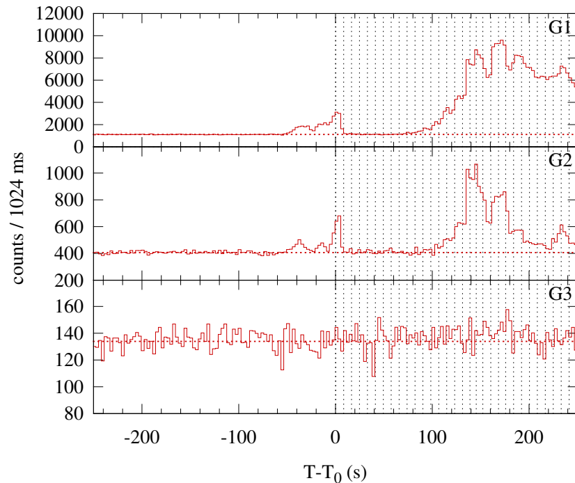
Konus-WIND S2 SOL2004-07-13T19:27 (M6.2) T_0 = 70032.248 s UT (19:27:12.248)
