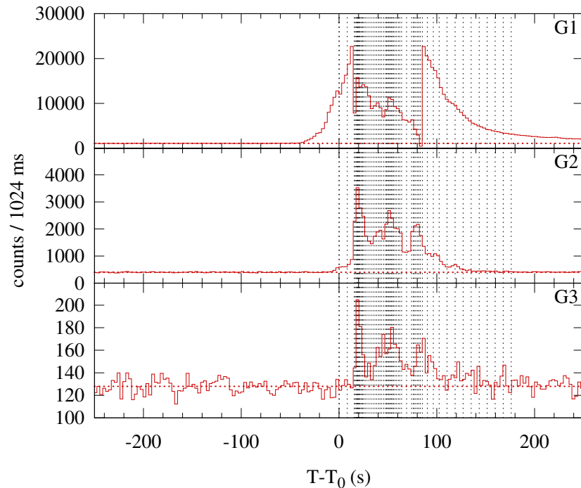
Konus-WIND S2 SOL2004-07-17T07:55 (X1.0) T 0 = 28508.884 s UT (07:55:08.884)
