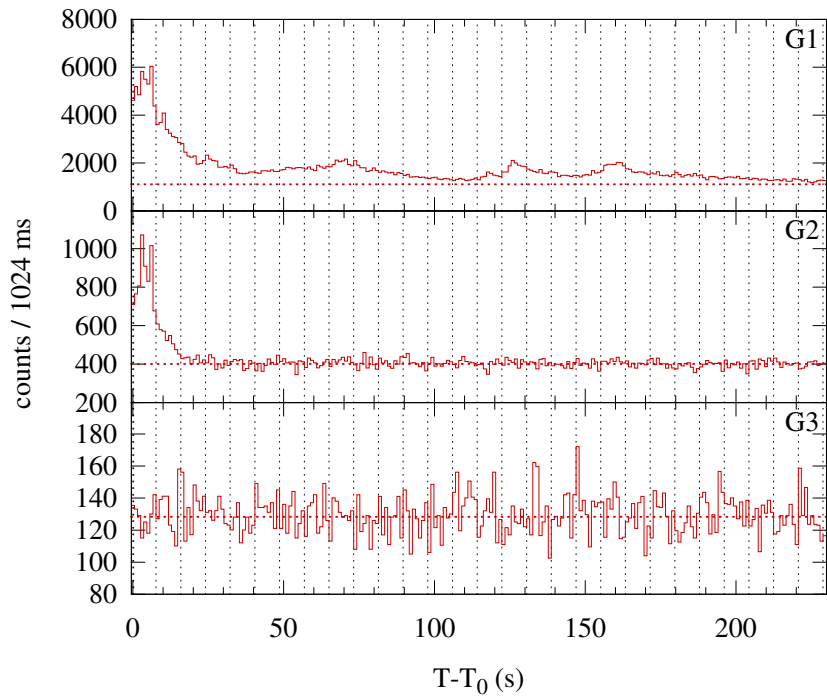
Konus-WIND S2 SOL2004-07-18T02:54 (M1.5) T 0 = 10441.450 s UT (02:54:01.450)
