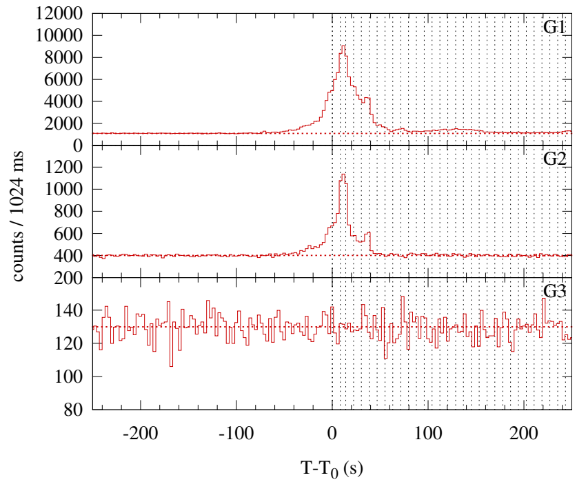
Konus-WIND S2 SOL2004-07-22T07:44 (C5.3) T_0 = 27850.372 s UT (07:44:10.372)
