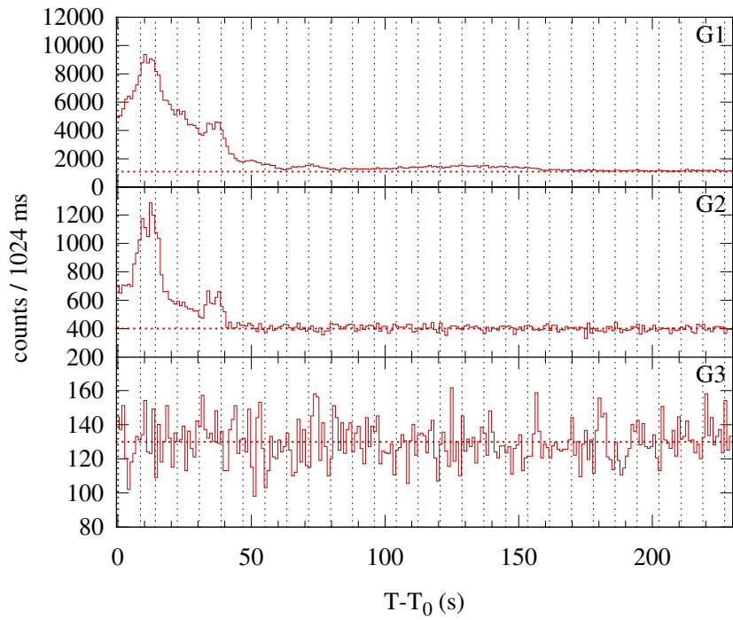
Konus-WIND S2 SOL2004-07-22T07:44 (C5.3) T_0 = 27850.372 s UT (07:44:10.372)
