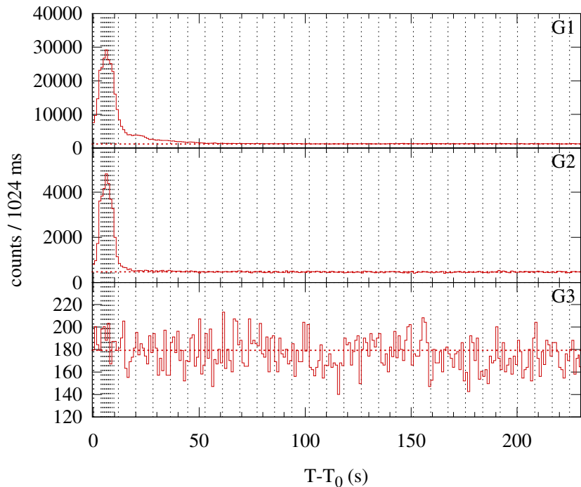
Konus-WIND S2 SOL2004-07-24T13:34 (C4.8) T 0 = 48869.869 s UT (13:34:29.869)
