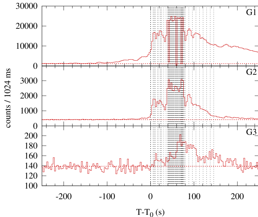
Konus-WIND S2 SOL2004-07-25T05:46 (M7.1) T_0 = 20793.755 s UT (05:46:33.755)
