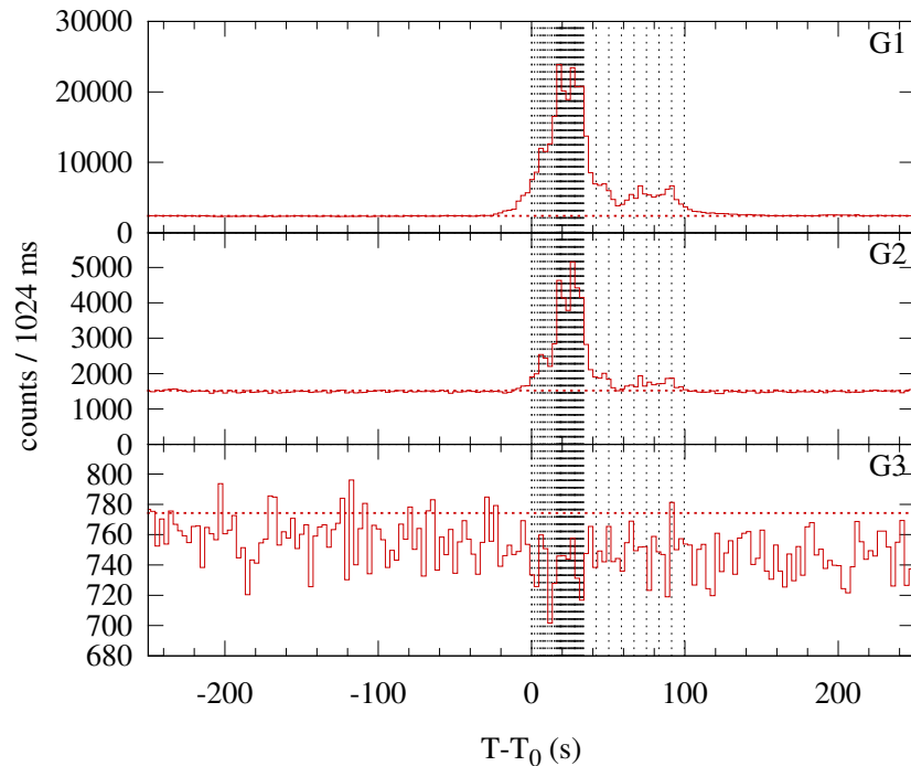
Konus-WIND S2 SOL2004-07-27T05:44 (M1.1) T_0 = 20656.961 s UT (05:44:16.961)
