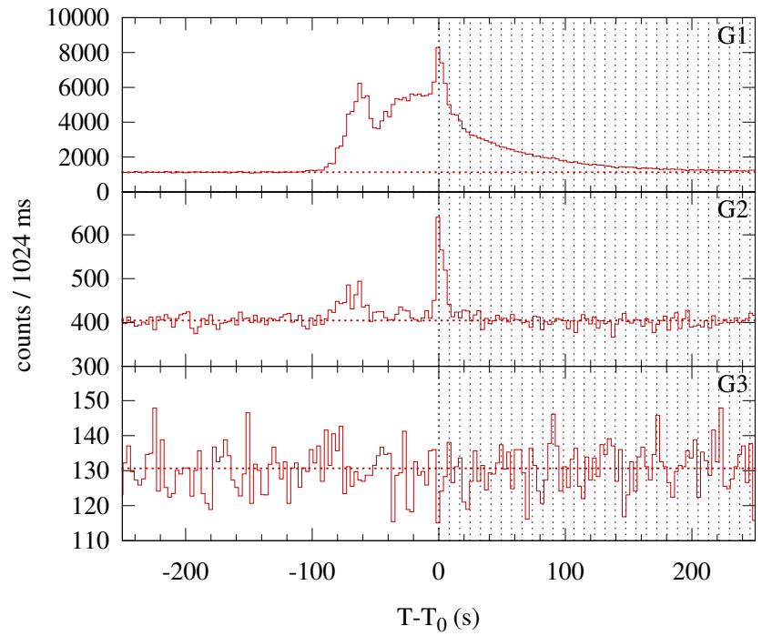
Konus-WIND S2 SOL2004-08-14T04:14 (M2.4) T_0 = 15244.207 s UT (04:14:04.207)
