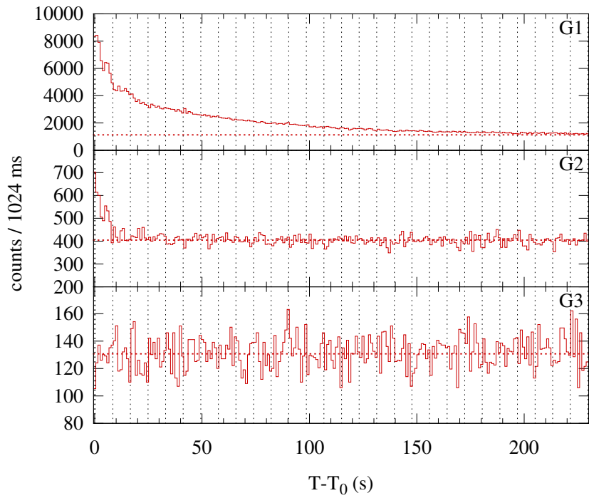
Konus-WIND S2 SOL2004-08-14T04:14 (M2.4) T_0 = 15244.207 s UT (04:14:04.207)
