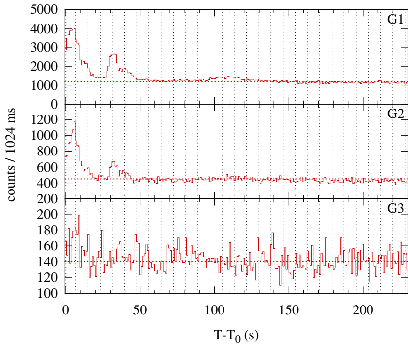
Konus-WIND S2 SOL2004-09-12T01:37 (M3.2) T_0 = 5824.470 s UT (01:37:04.470)
