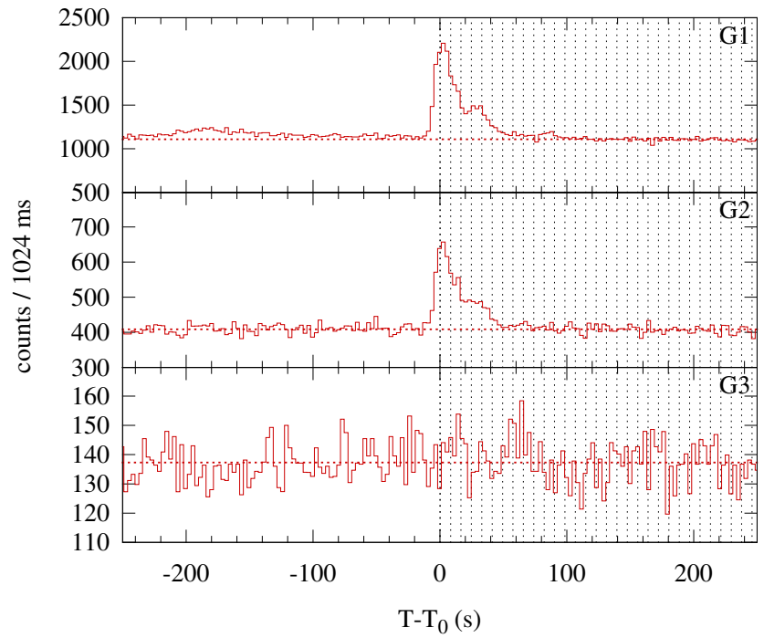
Konus-WIND S2 SOL2004-10-21T19:47 (C9.9) T_0 = 71237.300 s UT (19:47:17.300)
