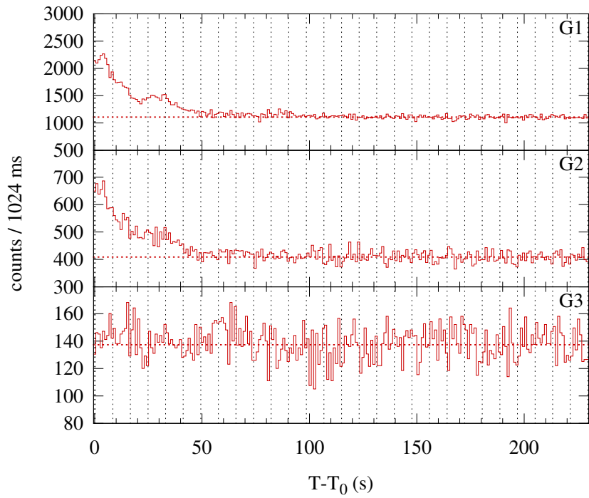
Konus-WIND S2 SOL2004-10-21T19:47 (C9.9) T_0 = 71237.300 s UT (19:47:17.300)
