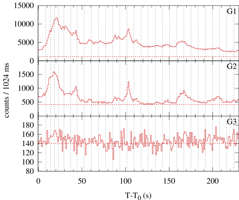
Konus-WIND S2 SOL2004-10-30T03:29 (M3.3) T_0 = 12579.971 s UT (03:29:39.971)
