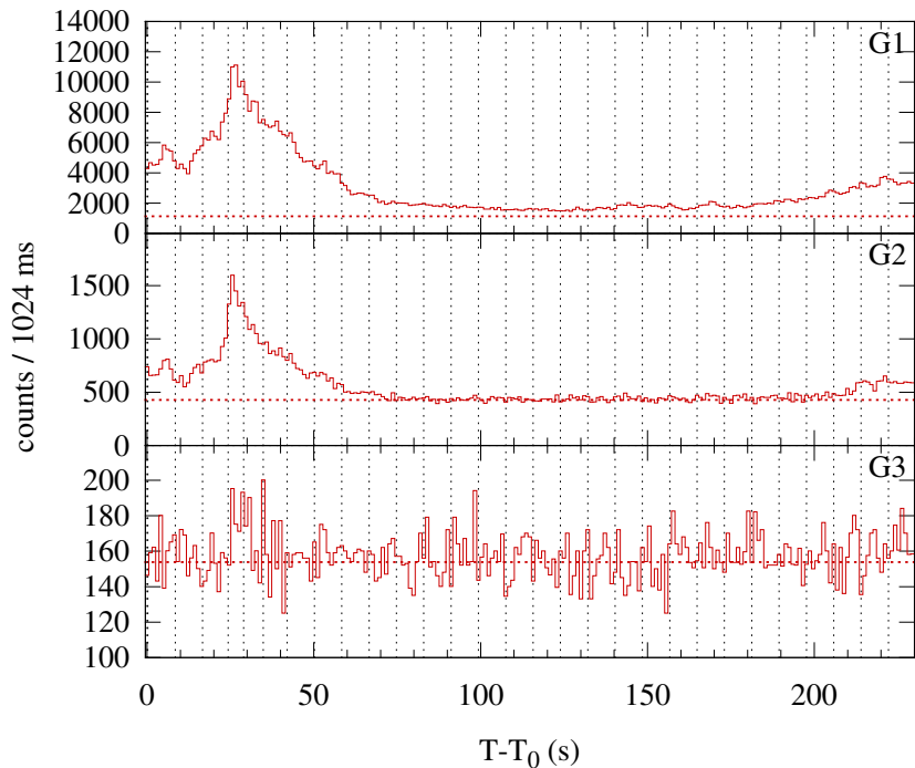
Konus-WIND S2 SOL2004-11-03T01:26 (M2.8) T 0 = 5203.205 s UT (01:26:43.205)
