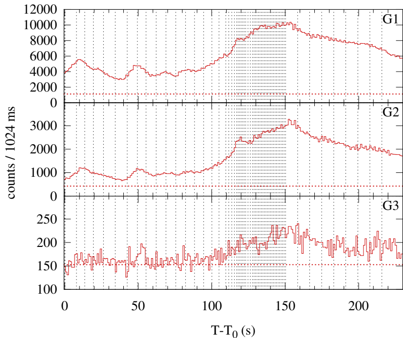
Konus-WIND S2 SOL2004-11-03T03:28 (M1.6) T_0 = 12510.983 s UT (03:28:30.983)
